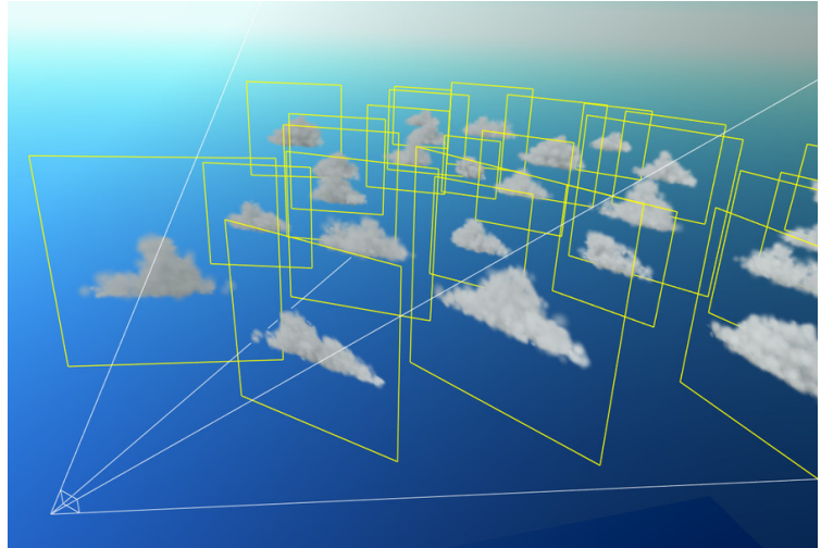
Figure 5: Impostors, outlined in this image, are textured polygons oriented toward the viewer.
