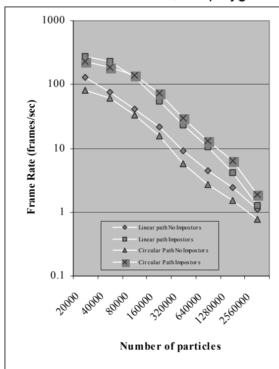
Figure 8: Results of performance measurements for cloudy scenes of varying complexity rendered with and without impostors.
