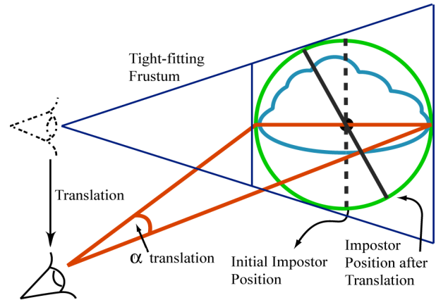
Figure 6: Impostor generation and translation error metric.
